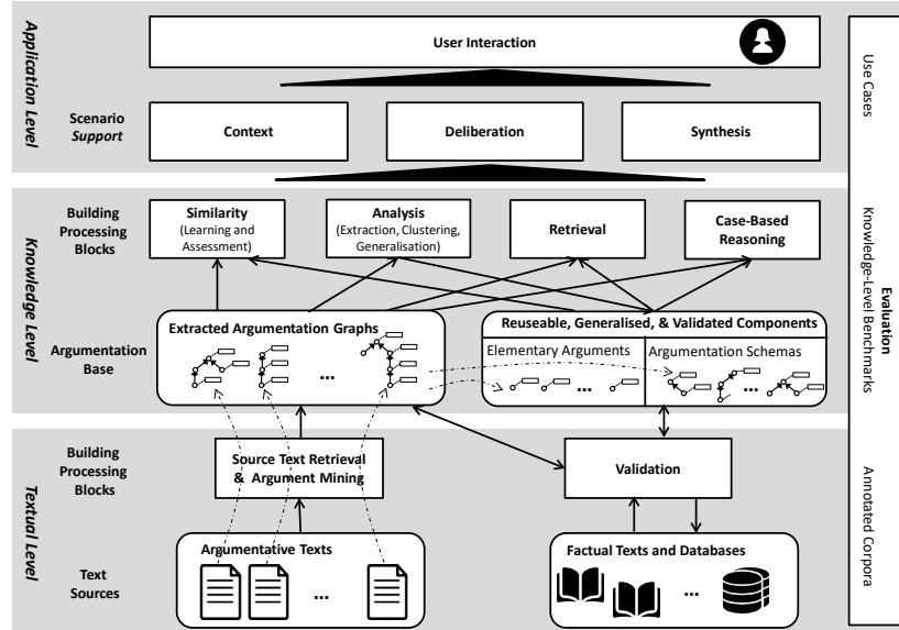
Fig. 1. Layered Architecture of the Envisioned Argumentation Machine
